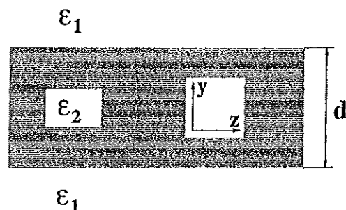
Figure 1. Symmetric-slab waveguide geometry.
